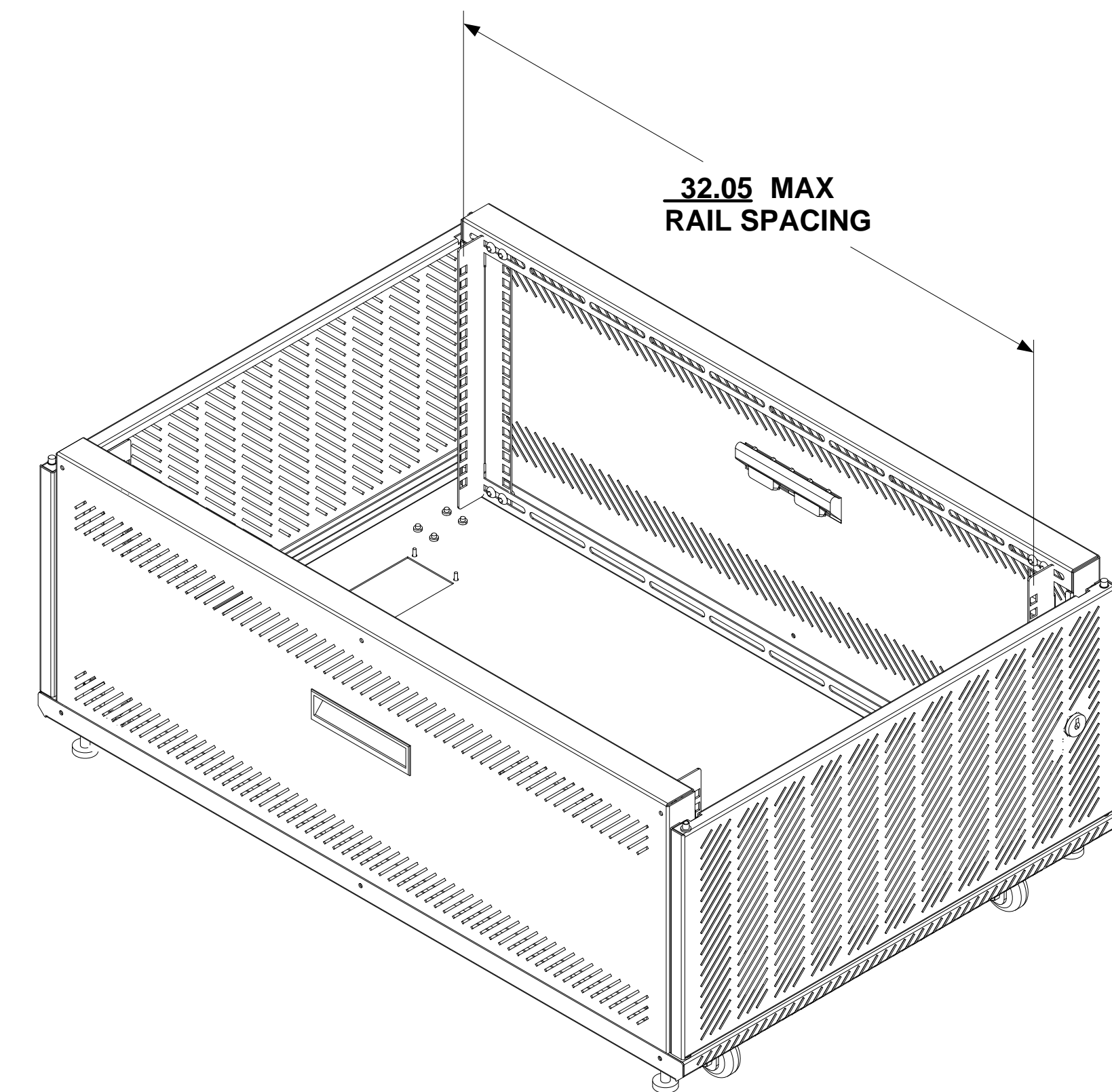
ISOMETRIC VIEW WITH TOP REMOVED
