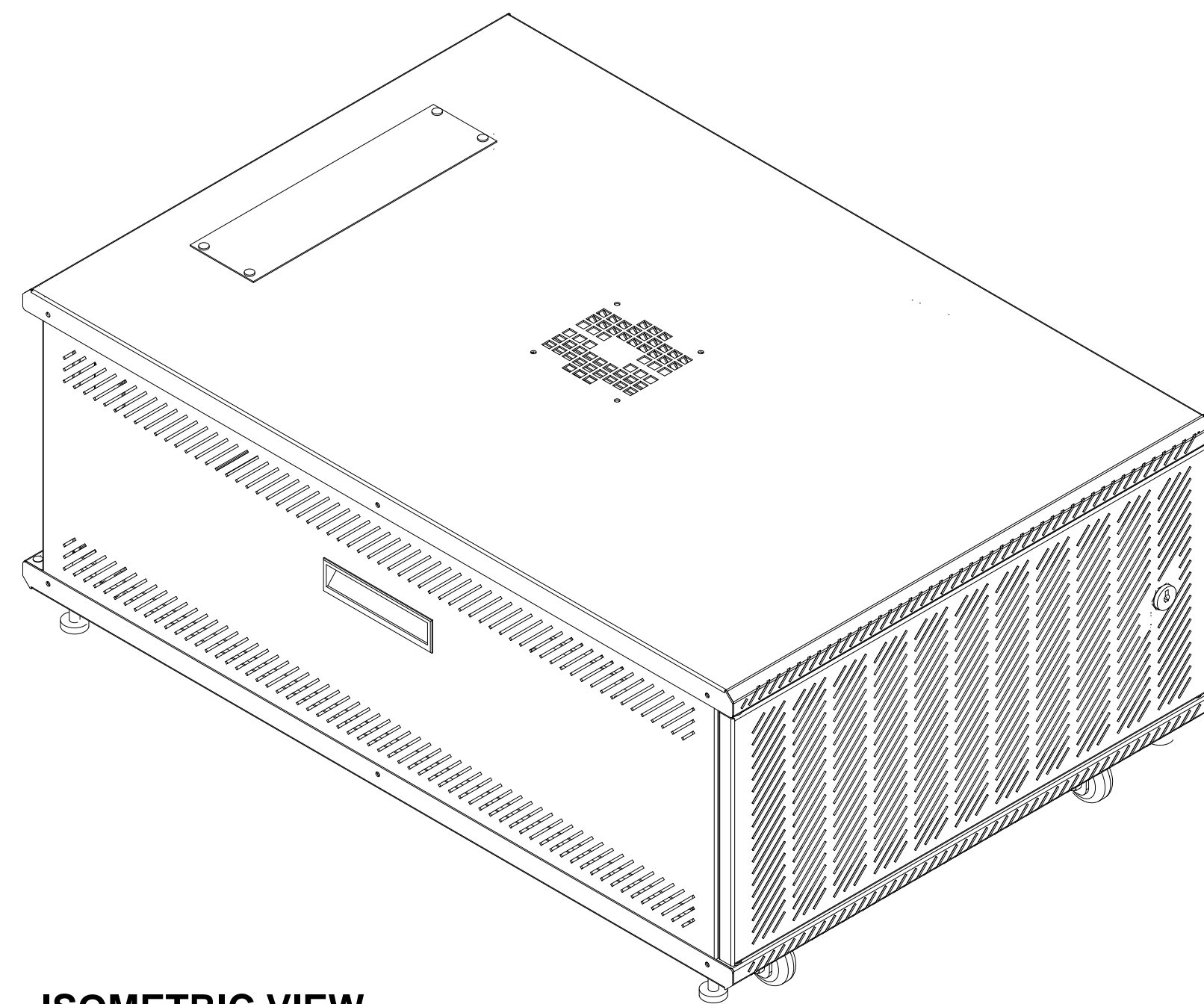
ISOMETRIC VIEW
