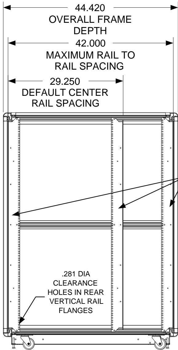
SIDE SECTION VIEW
