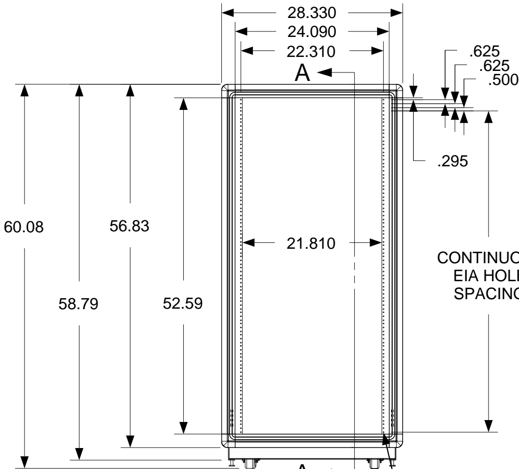
FRONT VIEW
