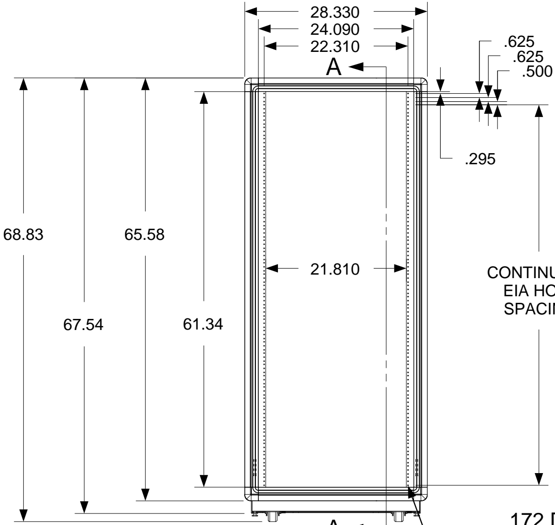
FRONT VIEW
