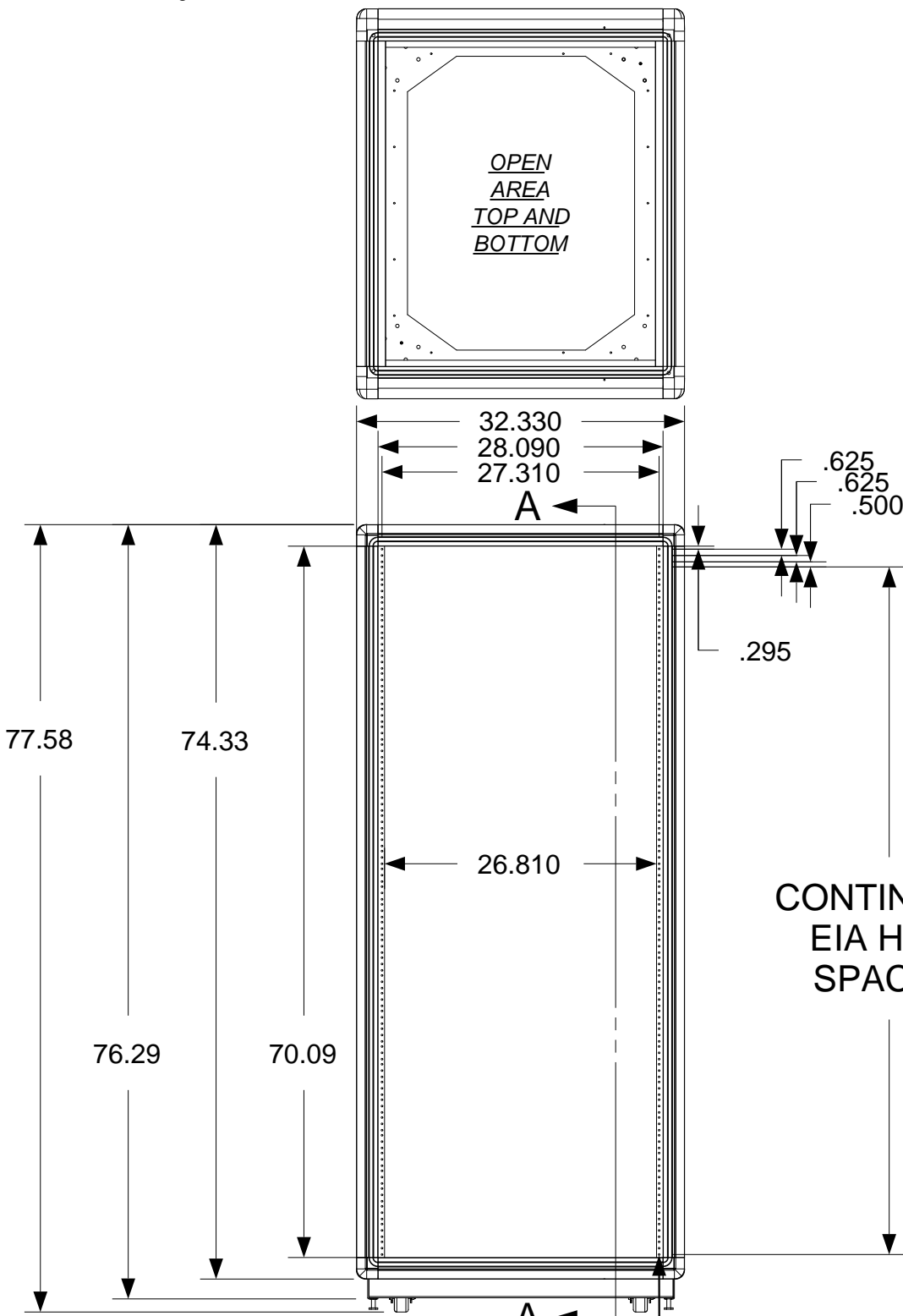
FRONT VIEW
