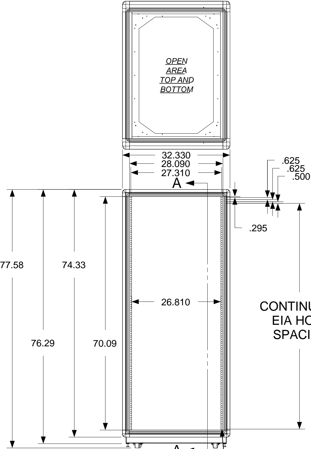
FRONT VIEW
